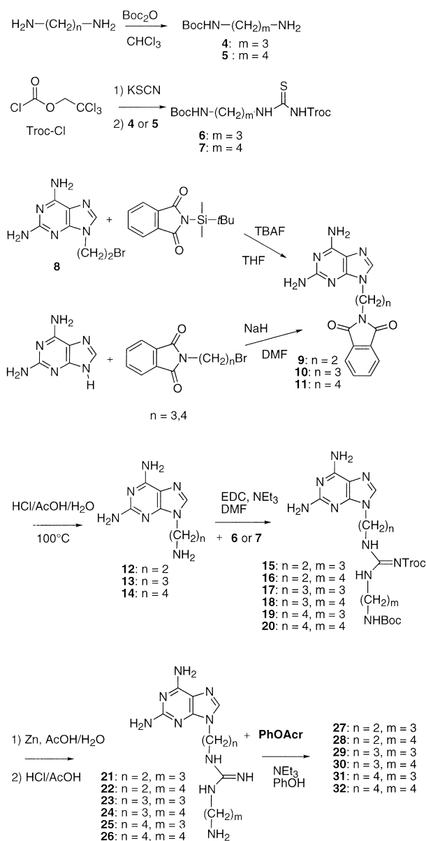
Scheme 1. Syntheses.
