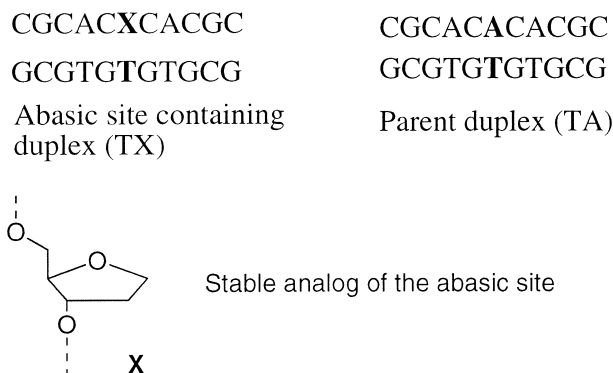
Scheme 2. Sequences of the synthetic oligonucleotides used in the T_m experiments.
