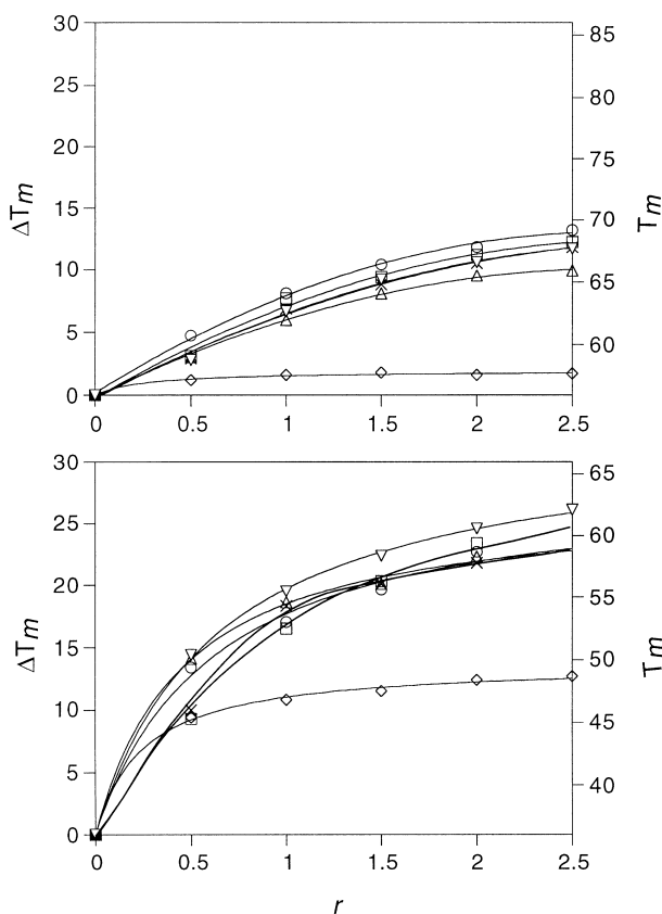
Figure 2. Influence of the drugs on the T_m and \Delta T_m of the TA (above) and TX (below) duplexes. Experiments were conducted at pH 7 (10 mM sodium phosphate, 1 mM EDTA, 20 mM NaCl). The drugs tested were (○) 27 , (□) 28 , (◇) 29 , (X) 30 , (Δ) 31 , and (▽) 32 . \Delta T_m is the difference between the T_m of the duplex in the presence of the drug and the T_m of the duplex alone. T_m values were measured for various ratios r of drugs ( r = [\text{drug}]/[\text{Duplex}] ).
